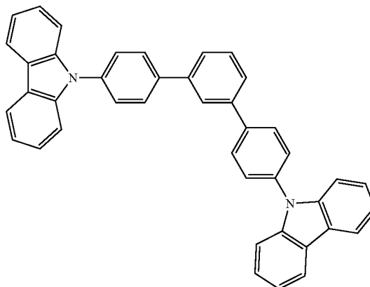
Compound (Comparative 3)
